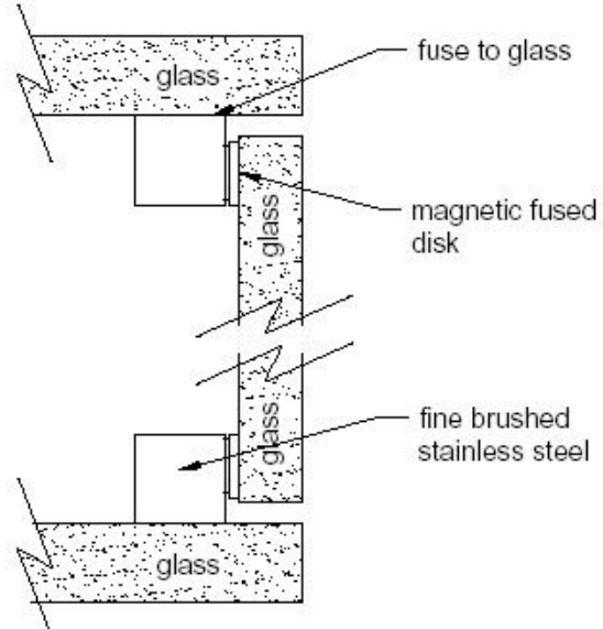
SECTION
